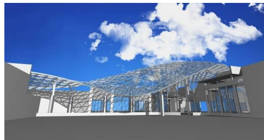
Fig. 3: Grasshopper generative model of Ballito Lifestyle Mall canopy imported into Archicad via Geometry Gym IFC translator
