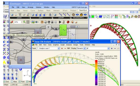
Fig. 2: Structural Analysis extraction from Grasshopper3d
